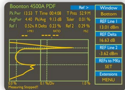
PDF of 8 carriers spaced 700 kHz apart from 1.8 GHz to 1.8049 GHz and phase aligned for highest peak power.
