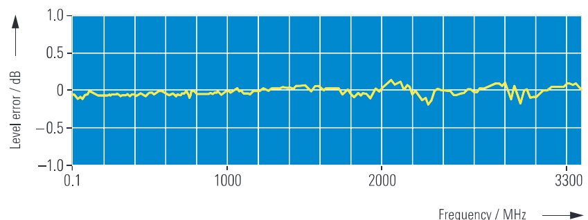
FIG 3 Typical level error at 0 dBm (SML03)
