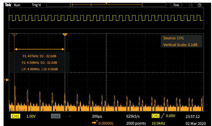
Figure 6: The time domain source waveform can be displayed above the FFT frequency spectrum
