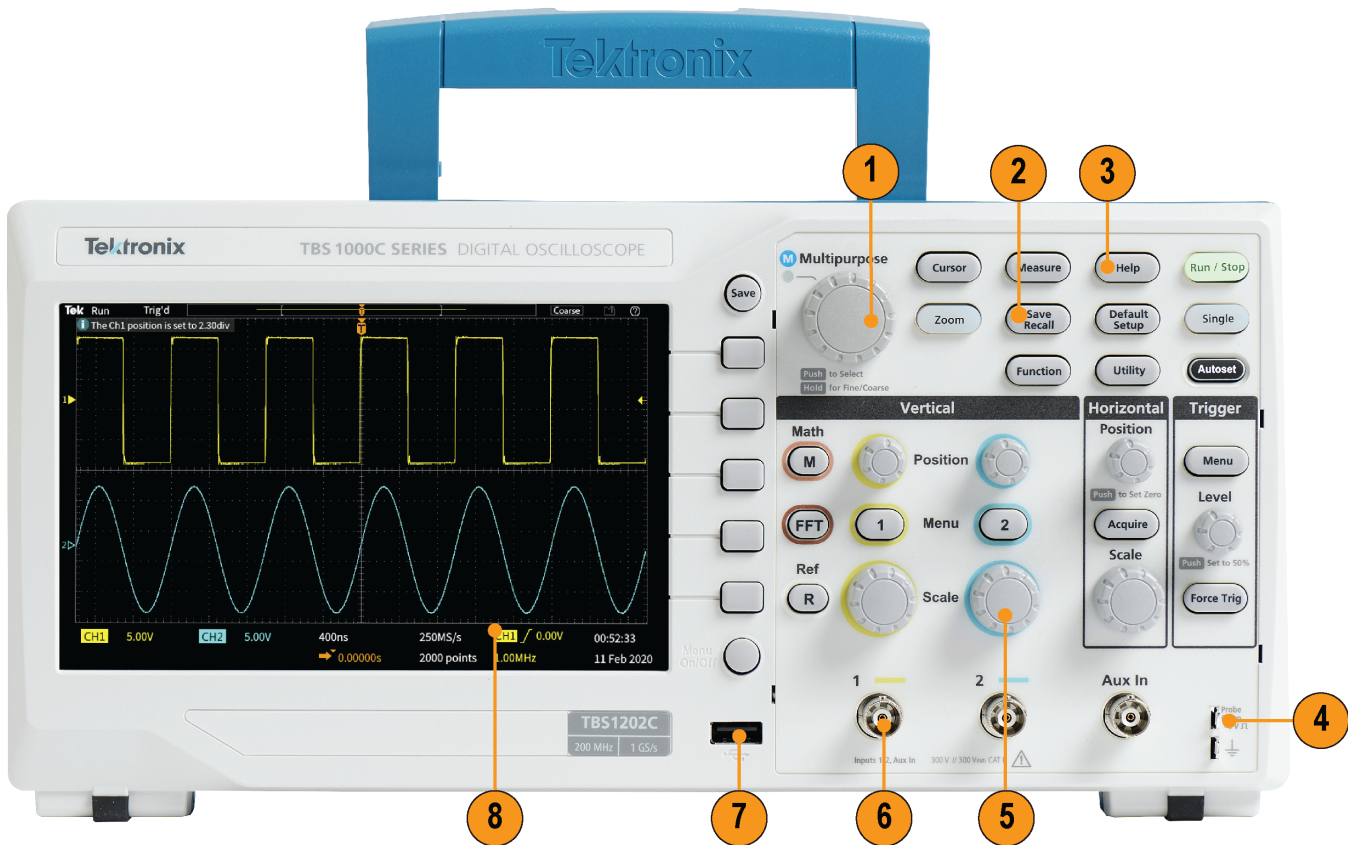
Figure 1: TBS1000C front panel
