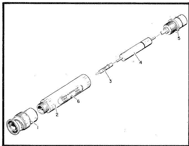
Figure 2. Model 10240B Parts
